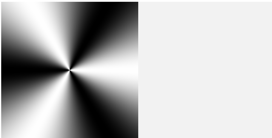
Figure 11.6: On the left, a grayscale representation of the function re^{i\theta} \mapsto \cos 3\theta . On the right, the uniform image used as a source for the Poisson editing.
