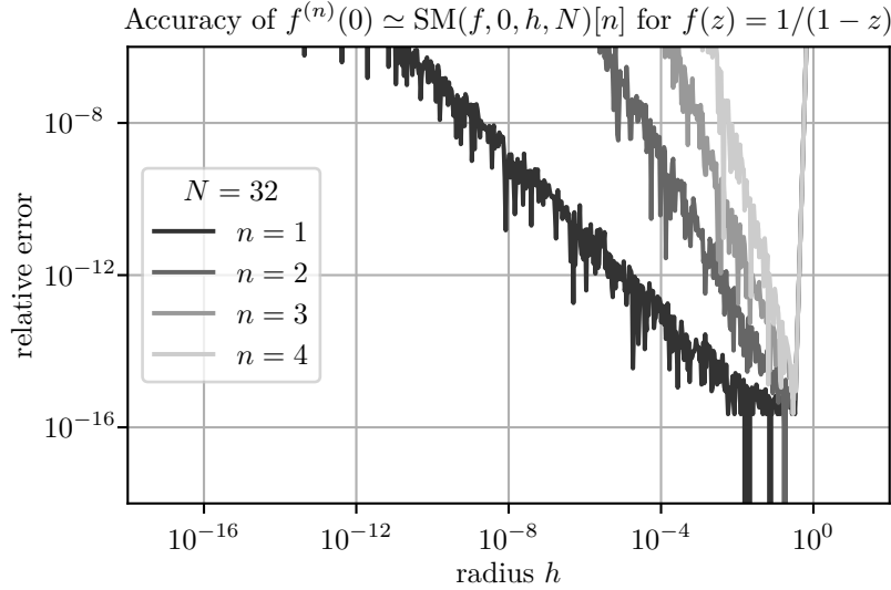
Figure 10.5: Spectral Method Error
