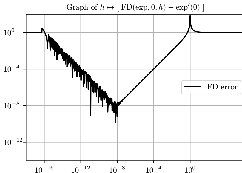
Figure 10.2: Forward Difference Scheme Error.
