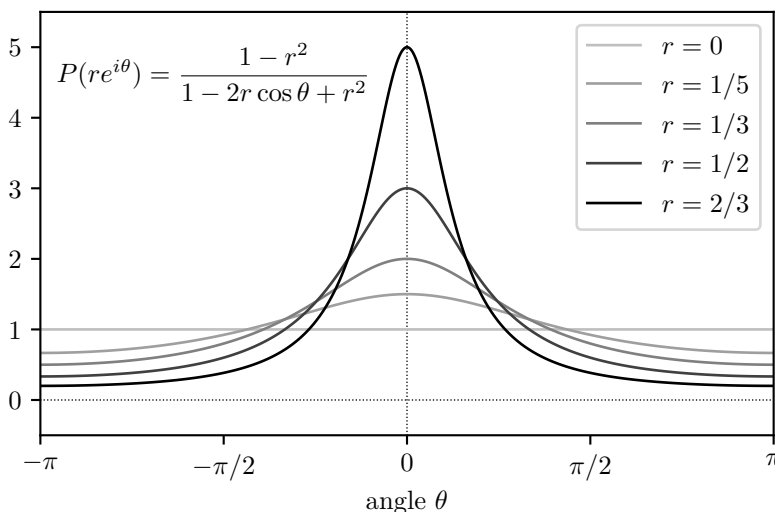
Figure 11.9: Poisson Kernel – Graphs of [\theta \mapsto P(re^{i\theta})]
