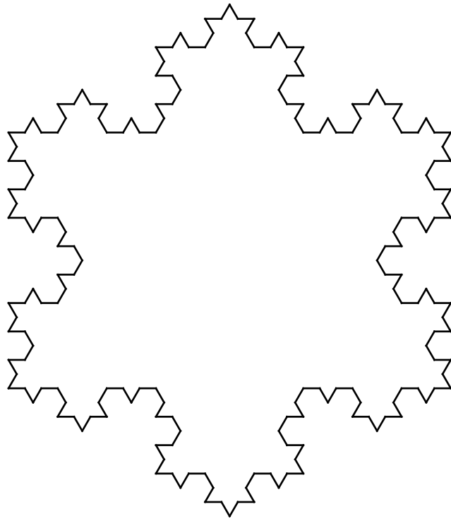
Figure 2.6: Image of the Koch snowflake, fourth iteration
