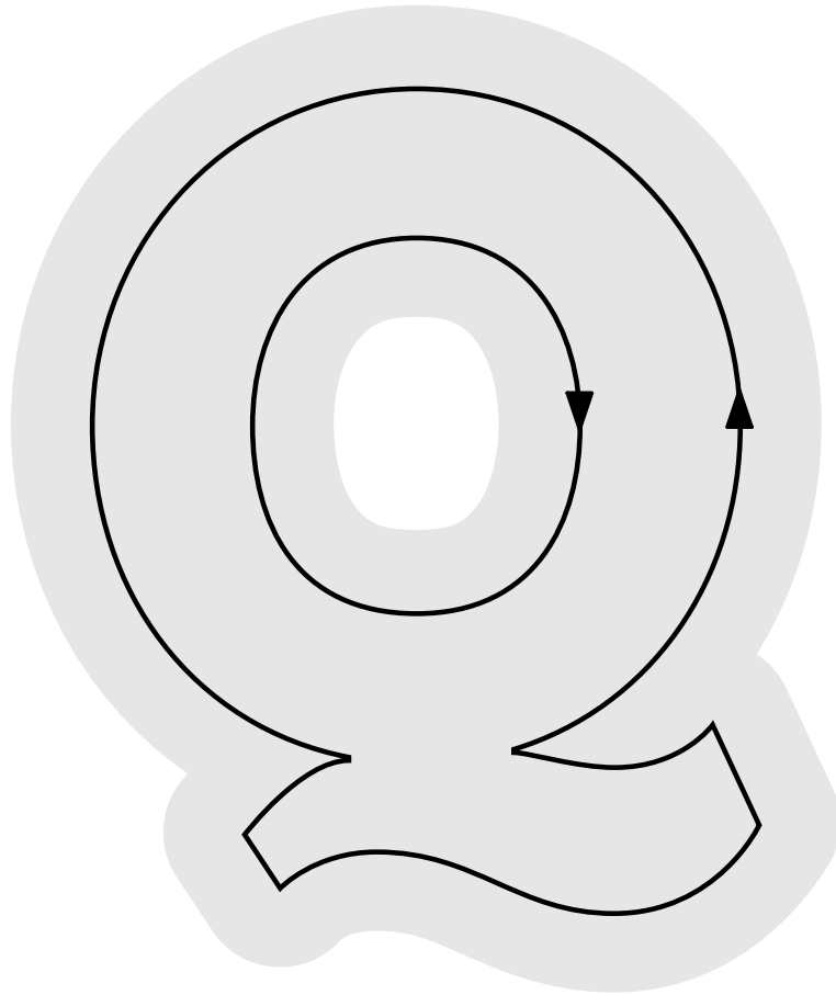
Figure 1: A pair \gamma of two rectifiable closed paths in an open set \Omega represented in light grey. Both paths are concatenations of quadratic Bézier curves.
