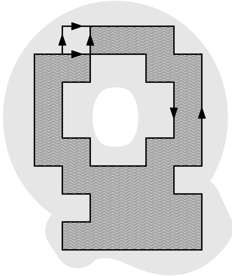
Figure 4: We can apply the local version of Cauchy's integral theorem "cell-by-cell" to such a path to prove the global version of the theorem.
